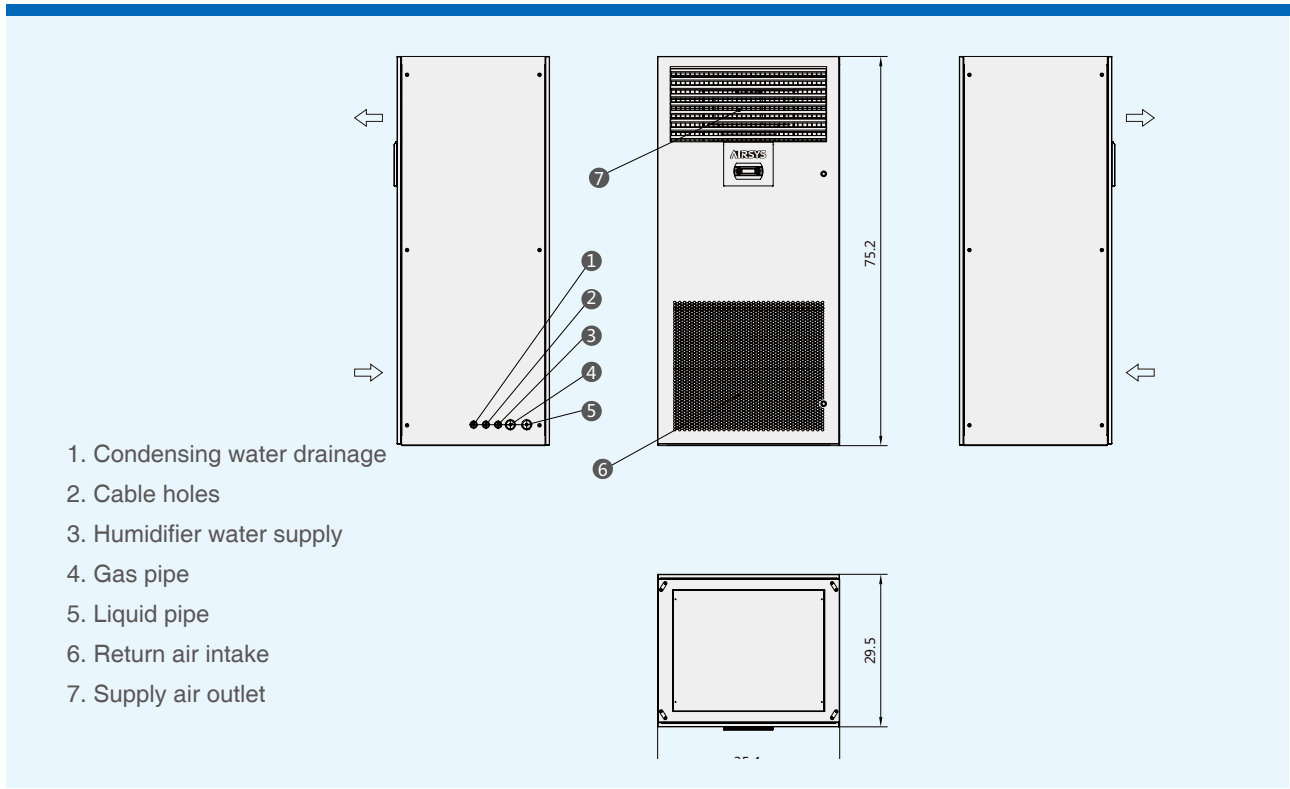
C2 Up-front throw (air) unit dimension drawing
