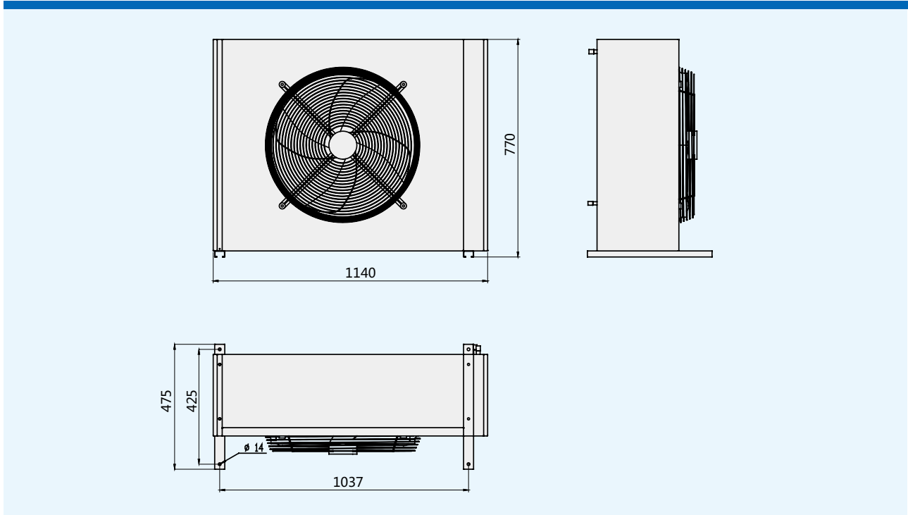
CMEG5 dimension drawing
