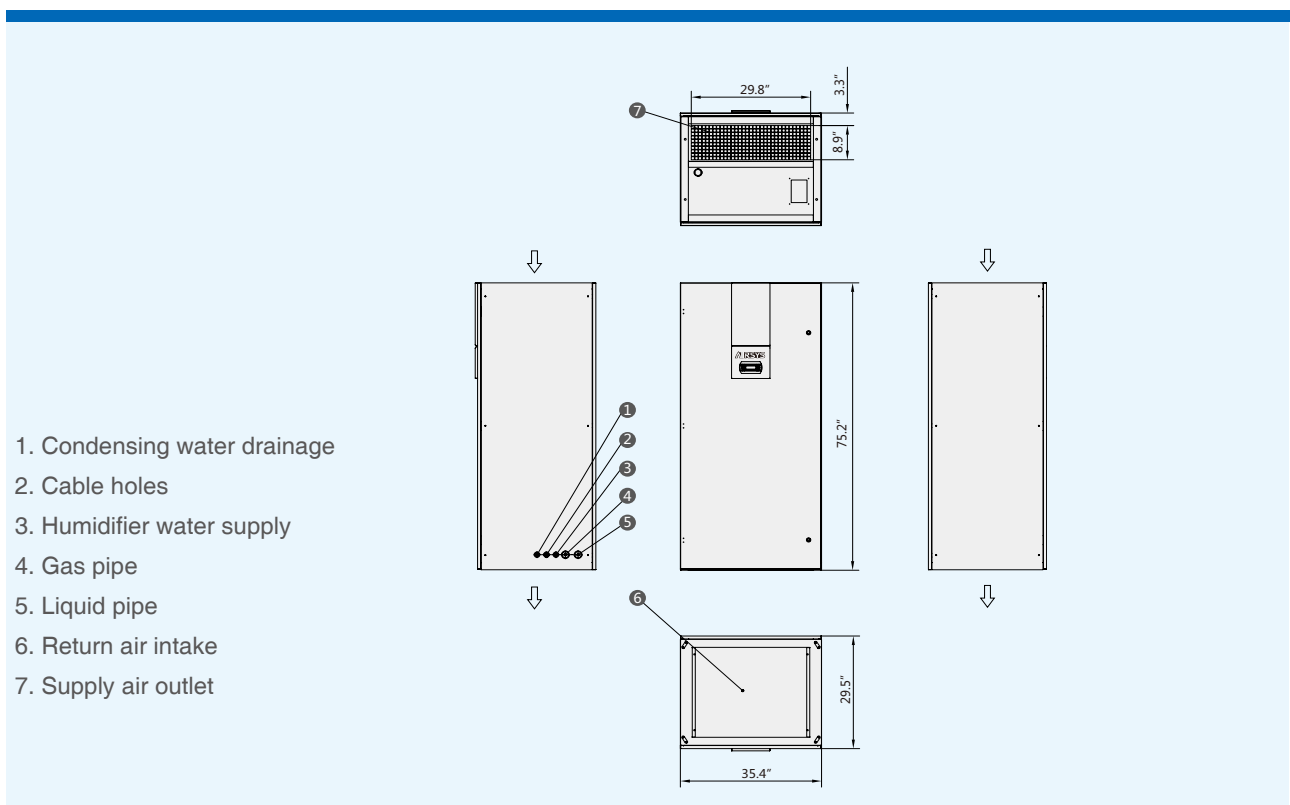
C2 Bottom throw (air) unit dimension drawing
